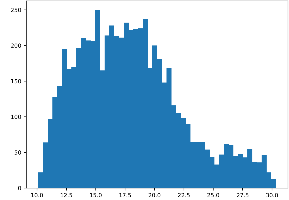
RT, n = 6338
