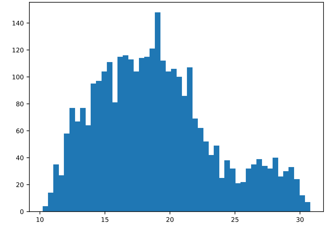
RT, n = 3228
