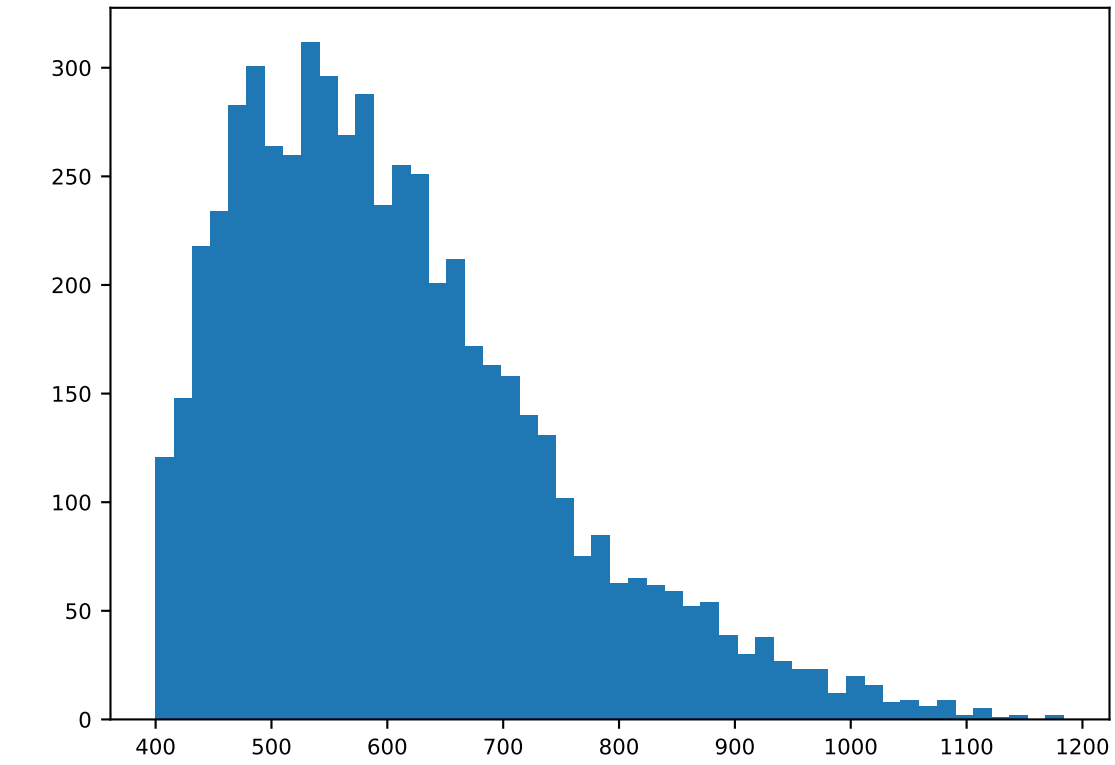
m/z, n = 5803
