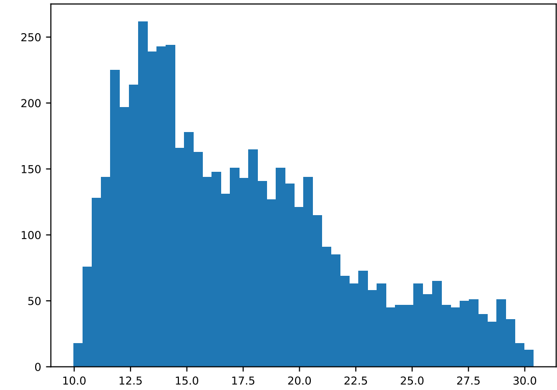
RT, n = 5526
