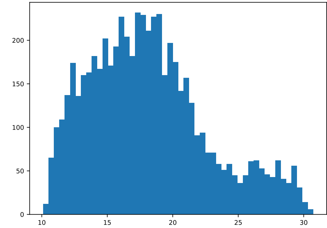
RT, n = 5803
