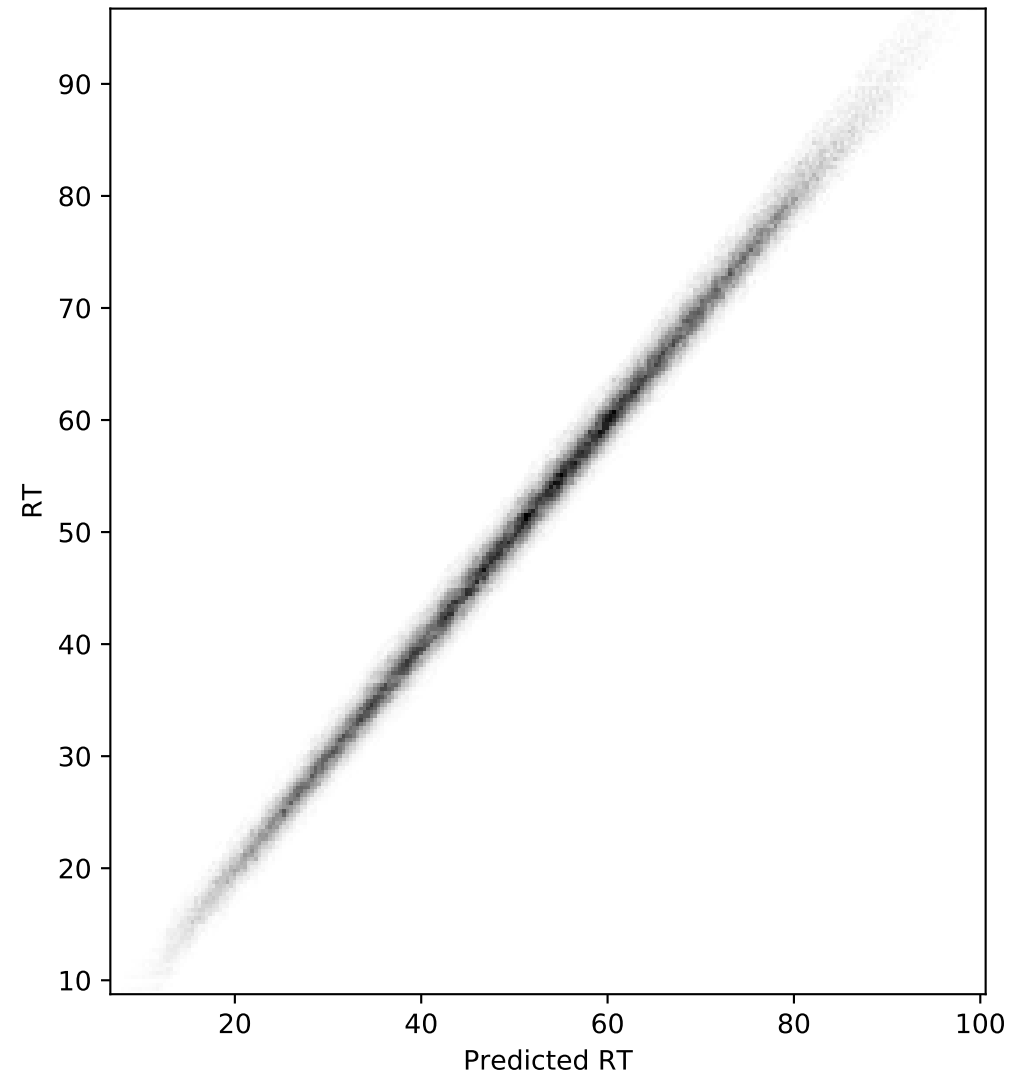
Retention time accuracy heatmap, all runs
