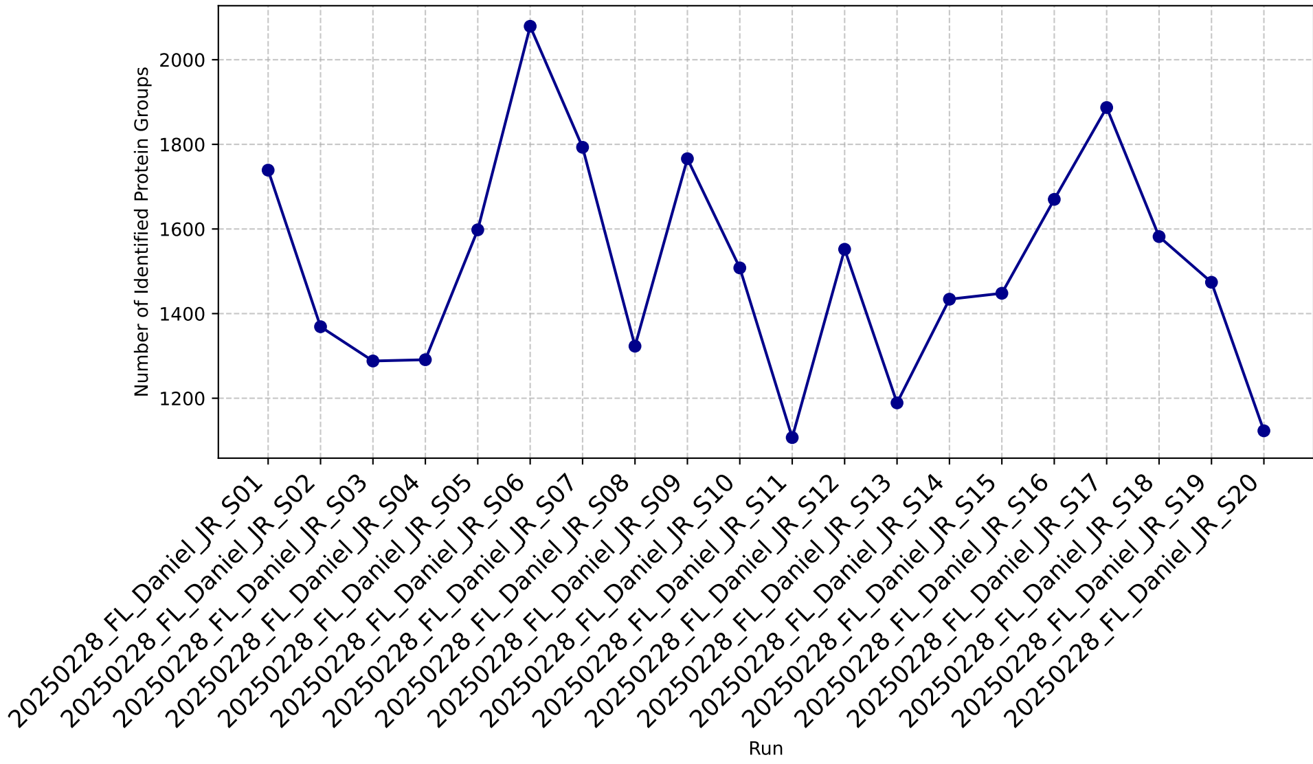
Number of Identified Protein Groups vs Run Order
