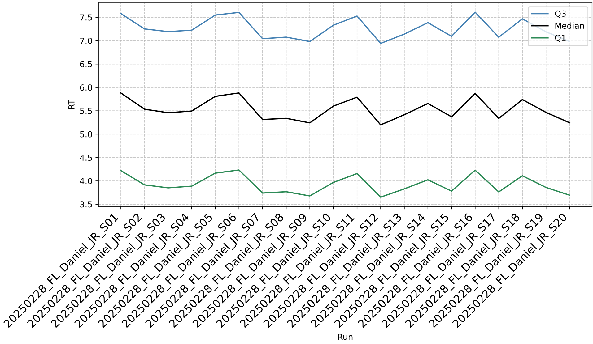
RT Distribution for Consistently Identified Precursors
