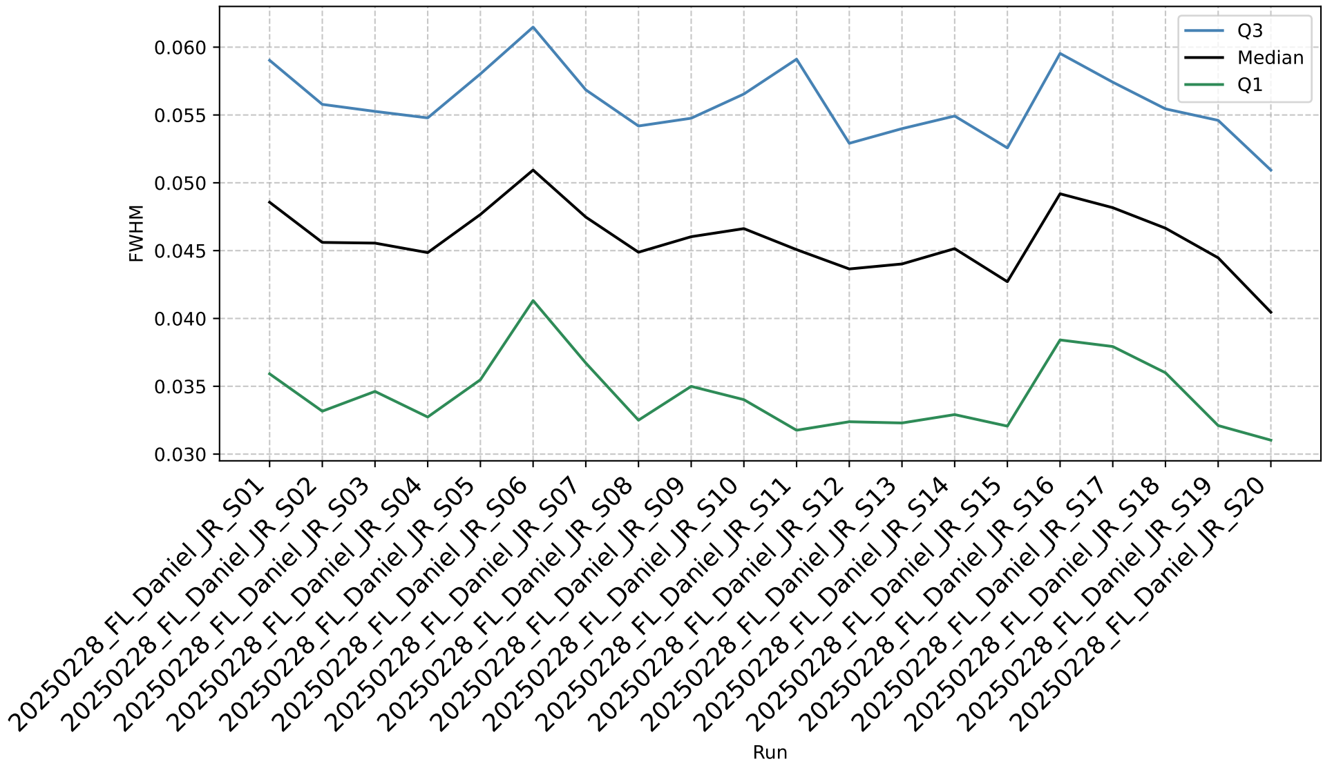
FWHM Distribution for Consistently Identified Precursors
